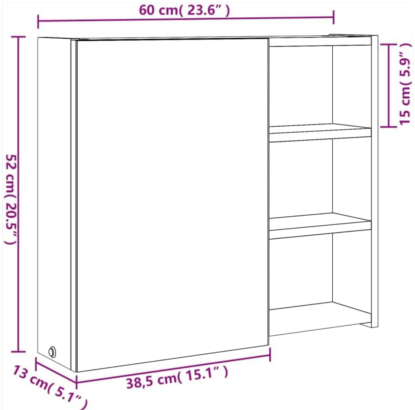
Image: Detailed dimensions of the cabinet for planning installation space.
