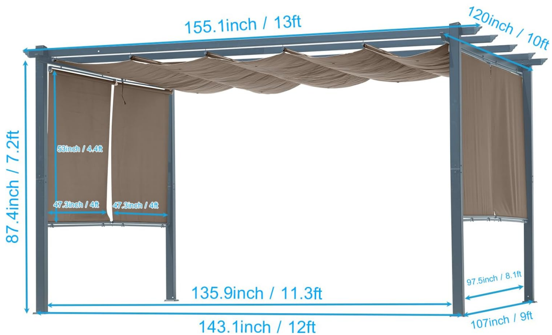
Figure 2.1: Product Dimension Drawing. This diagram provides detailed measurements of the pergola, indicating its overall length of 155.1 inches (13 ft), width of 120 inches (10 ft), and height of 87.4 inches (7.2 ft). It also shows dimensions for the side curtains and internal spacing.
