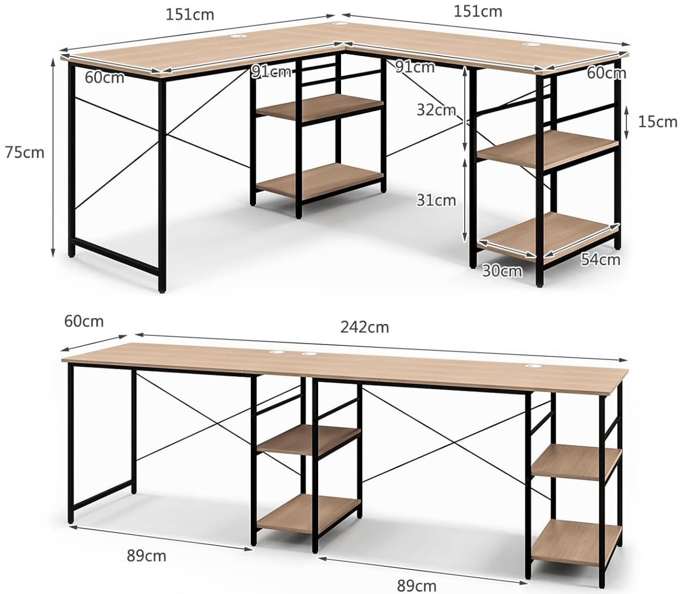
Figure 4.2: Two ways to assemble the desk.
