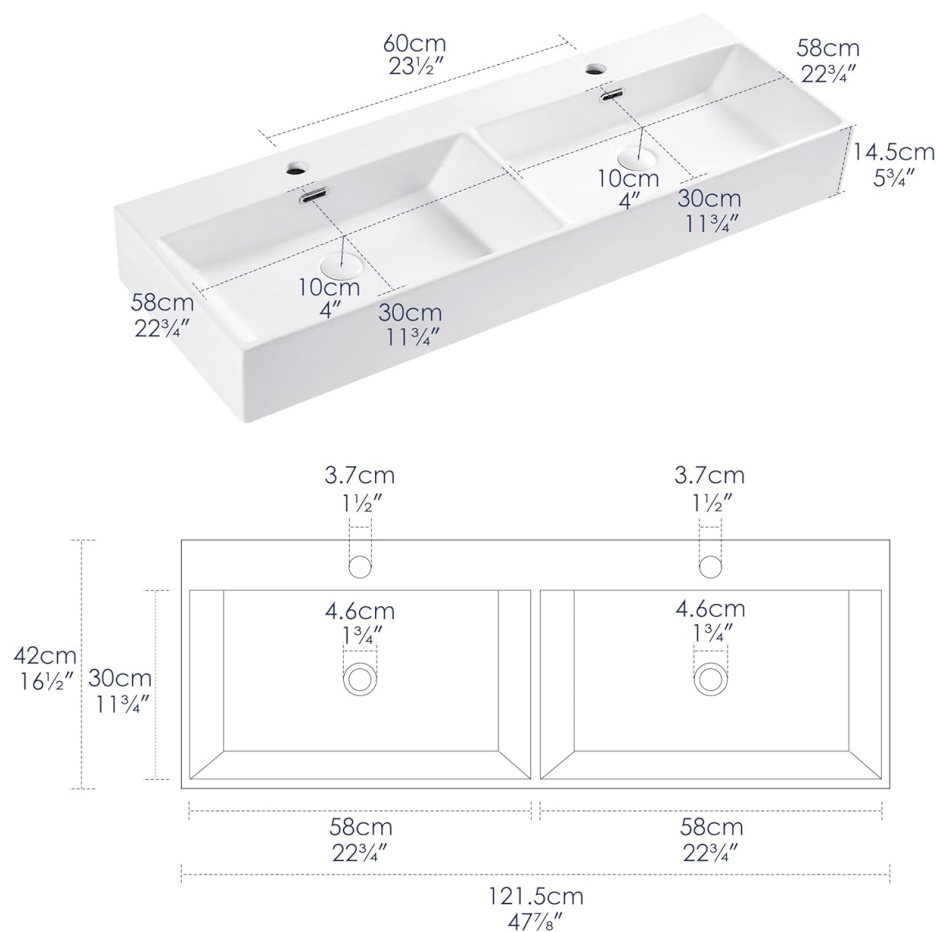
Image 4.1: Detailed technical dimensions of the Eridanus double bowl sink.
