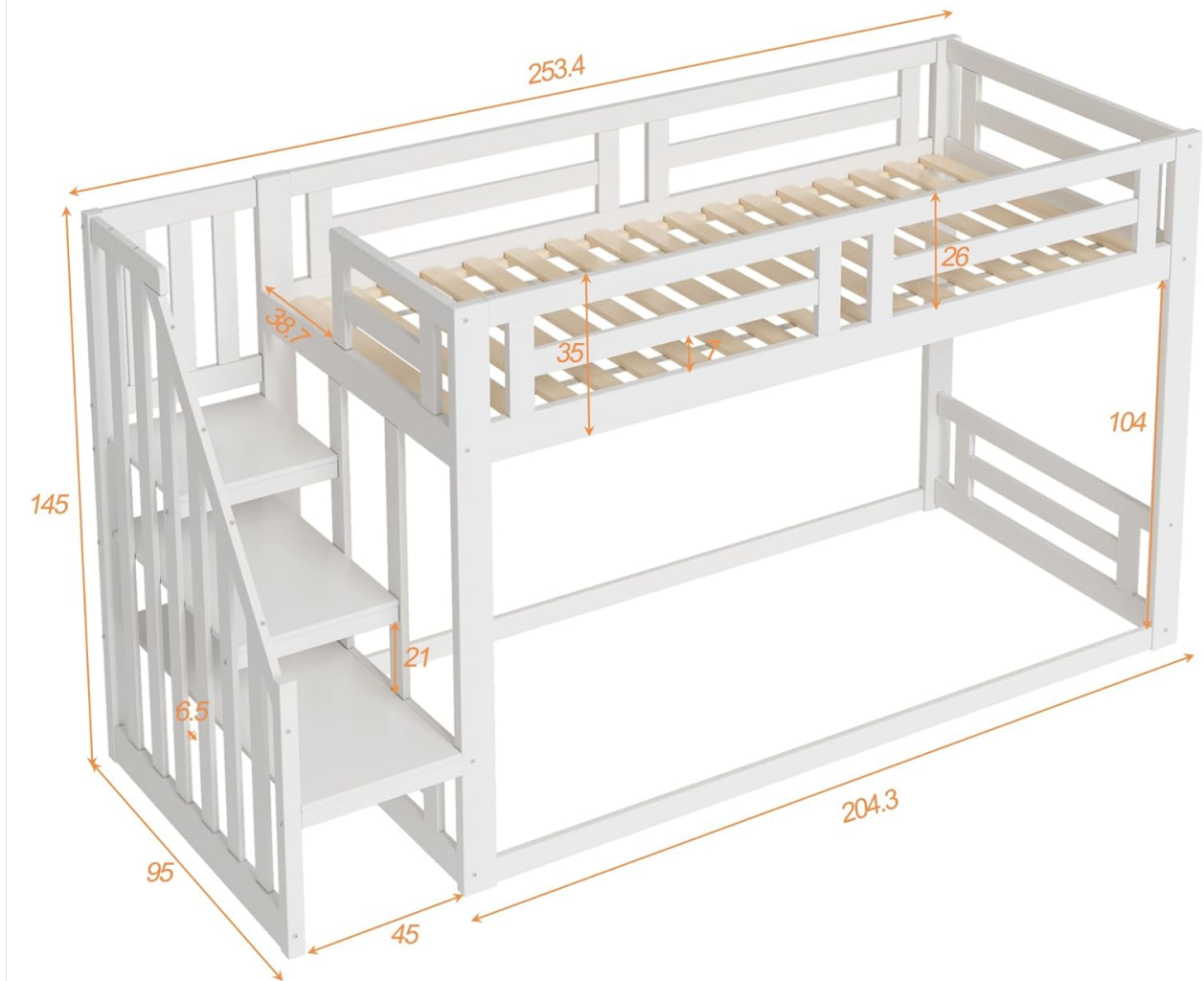
Figure 4.2: Dimensional overview of the bunk bed, showing length, width, and height measurements in centimeters.
