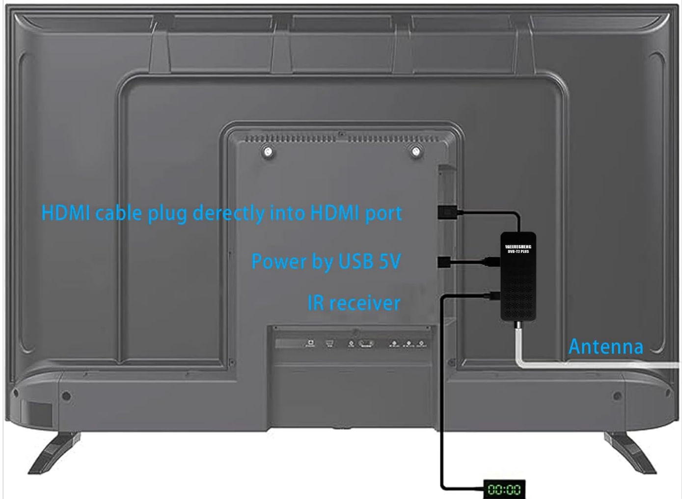
Image 5.2: The decoder unit connected and hidden behind a television, with the HDMI cable plugged directly into the TV and the IR receiver extended for remote control functionality. Power is supplied via a TV's USB port.
