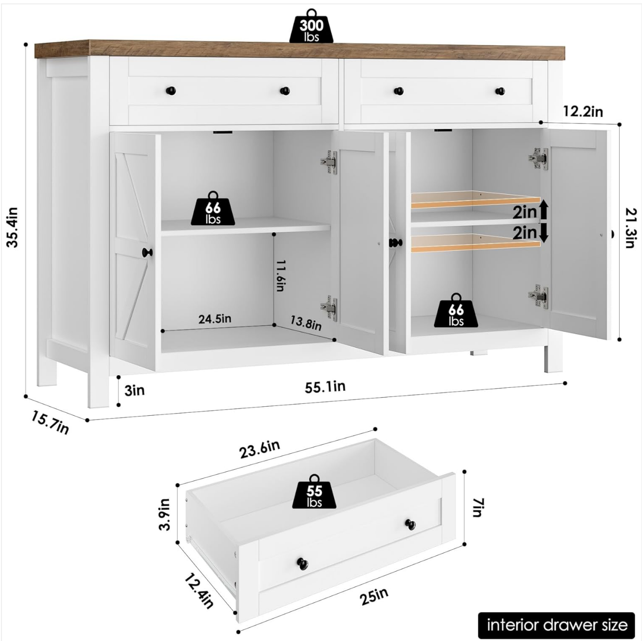
Figure 4.2: Dimensions and weight capacities for the cabinet, shelves, and drawers.
