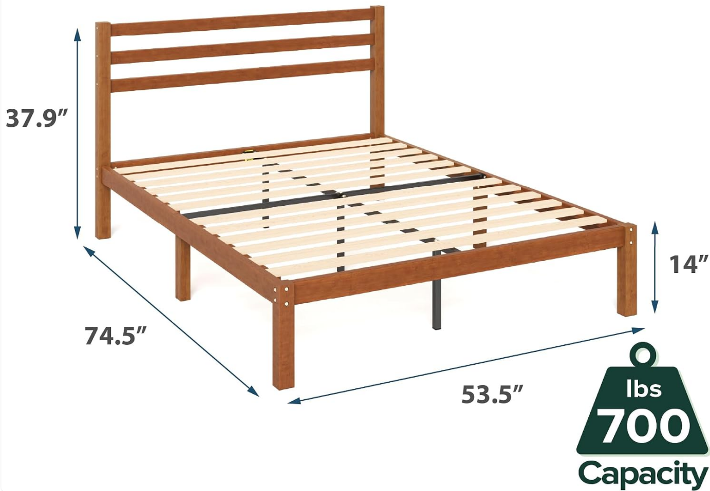
Image: A diagram illustrating the dimensions of the bed frame (74.5" L x 53.5" W x 37.9" H, 14" frame height) and its 700 lbs weight capacity.
