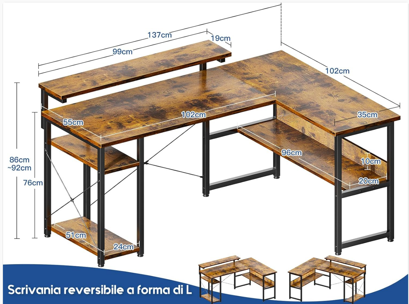
Figure 3.1: Dimensional diagram and illustration of the reversible L-shape assembly options.
