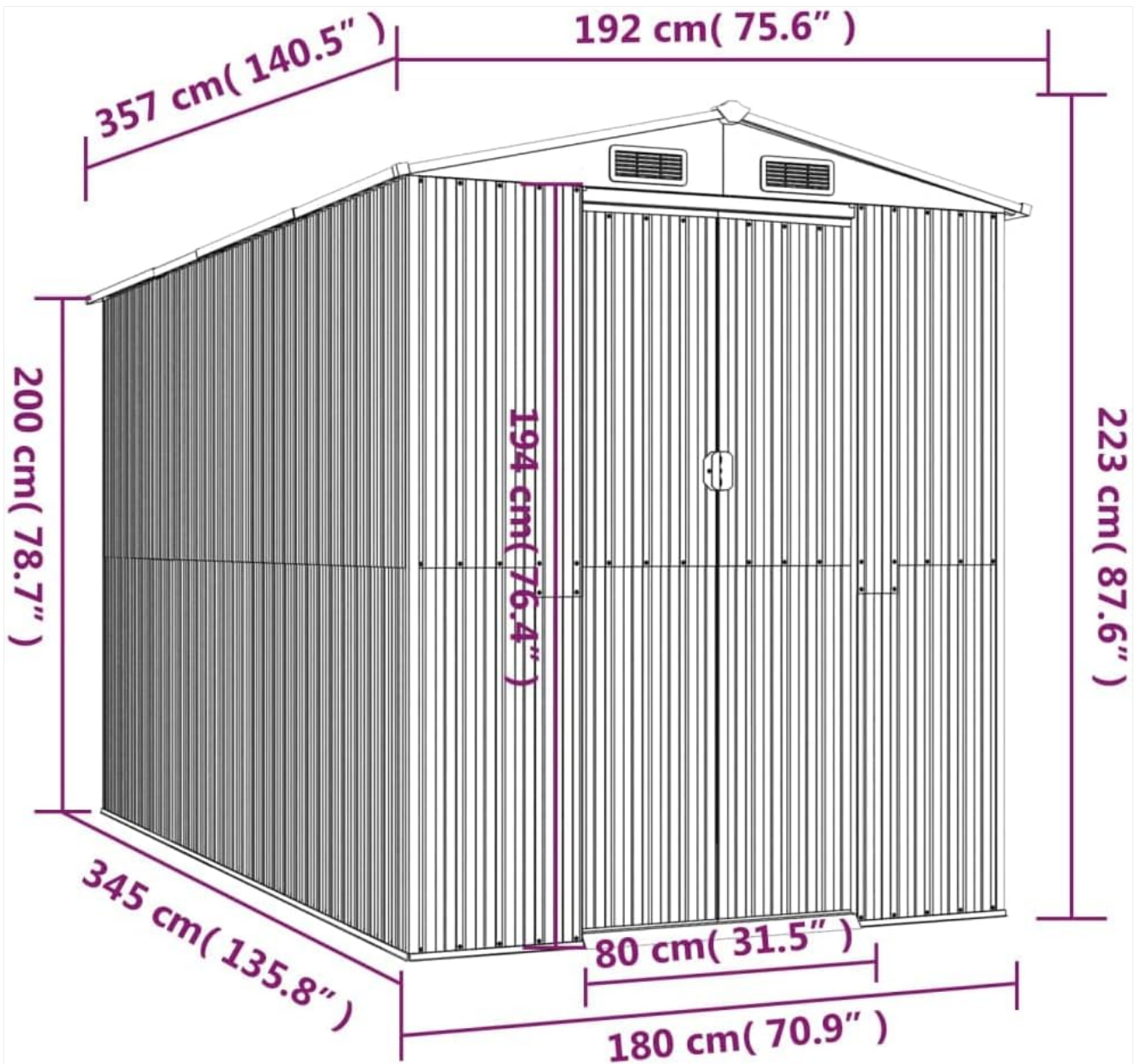
Image 6: Dimensional diagram of the shed, indicating width, length, and height measurements in both inches and centimeters.
