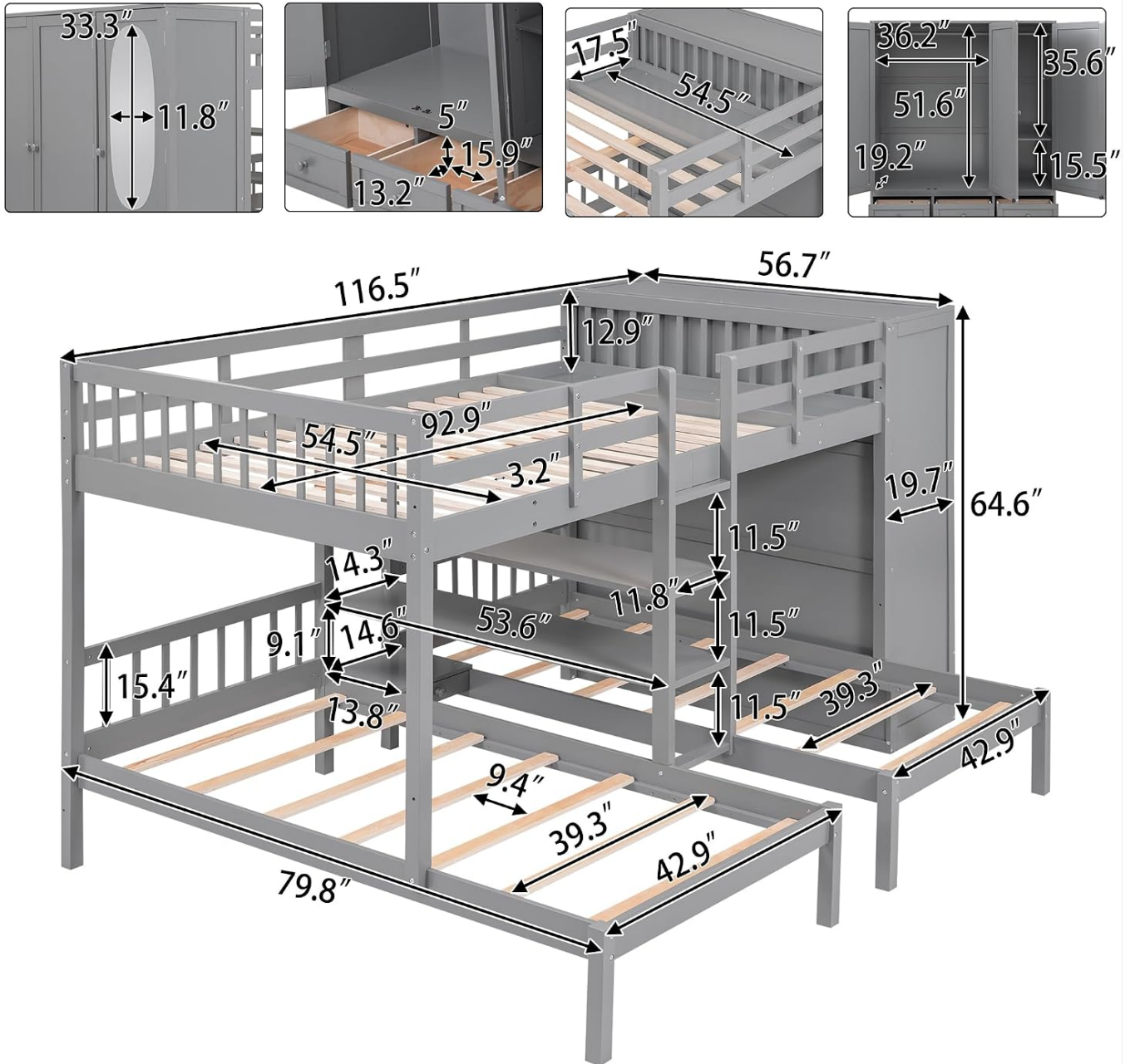
Image 4.1: Detailed dimensions of the bunk bed, wardrobe, and shelves, crucial for planning placement and assembly.
