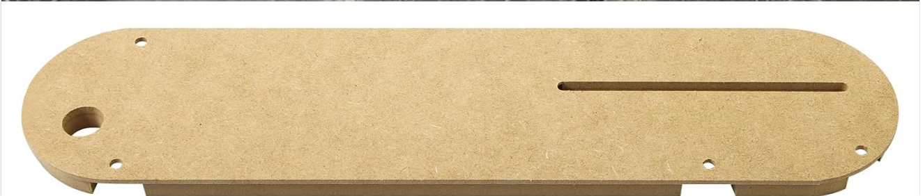
Figure 5.1: The Dado Throat Plate in action, demonstrating its effectiveness in reducing tear-out during cuts.
