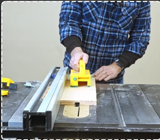
Figure 5.2: Proper technique for using the Dado Zero Gap Blade with the insert for precise cuts.
