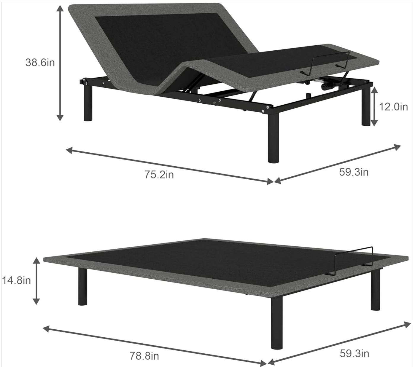
Figure 4.1: Dimensions of the adjustable bed frame.
