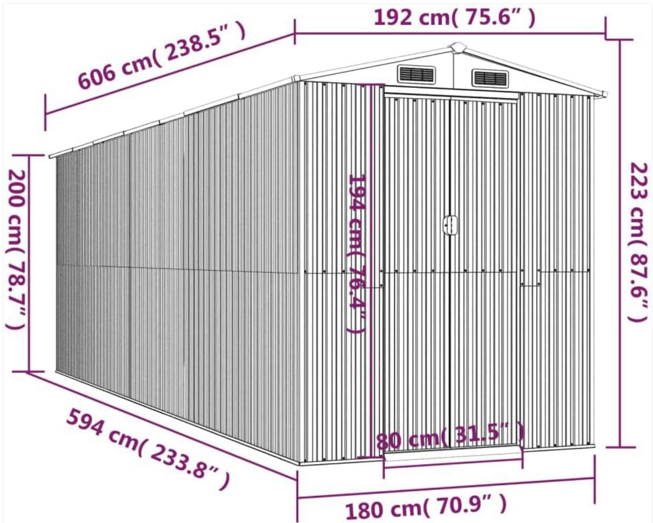
Image 4: A technical diagram illustrating the key dimensions of the vidaXL Galvanized Steel Garden Shed, including width, depth, and height measurements in both inches and centimeters.
