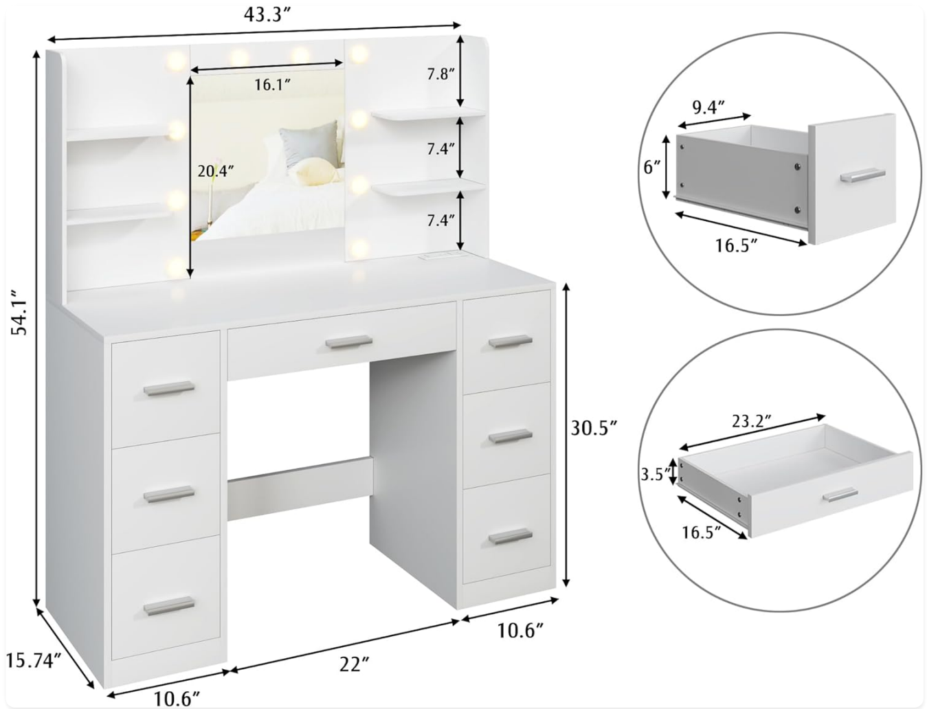
Figure 2: Product dimensions and general component layout.
