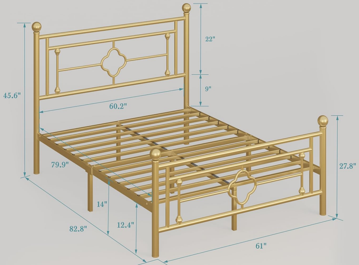
Figure 1: Queen Size Bed Frame Dimensions and Specifications.
