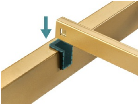
Figure 3: U-shaped Groove for quick and sturdy assembly.
