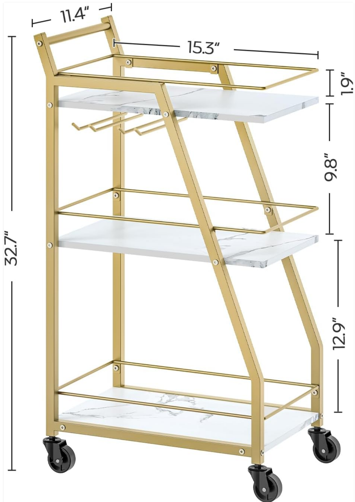
Image: Detailed dimensions of the YATINEY Bar Cart, illustrating its overall size and tier spacing.
