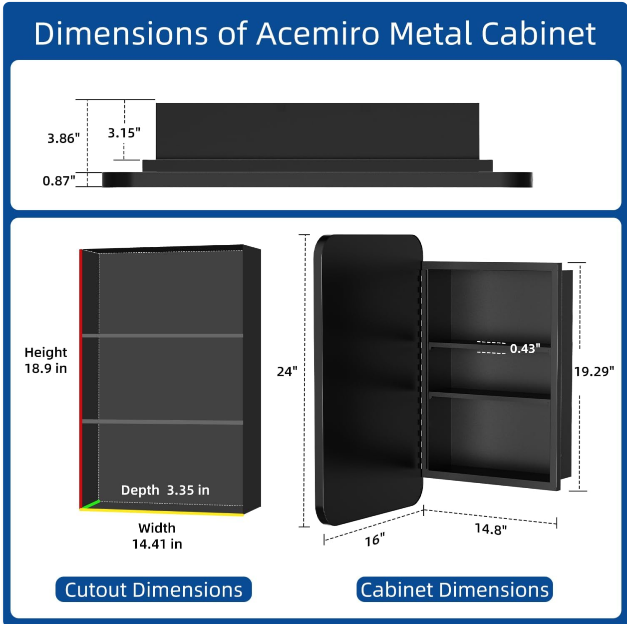
Image: Detailed dimensions for the ACEMIRO medicine cabinet and its required cutout for recessed installation.
