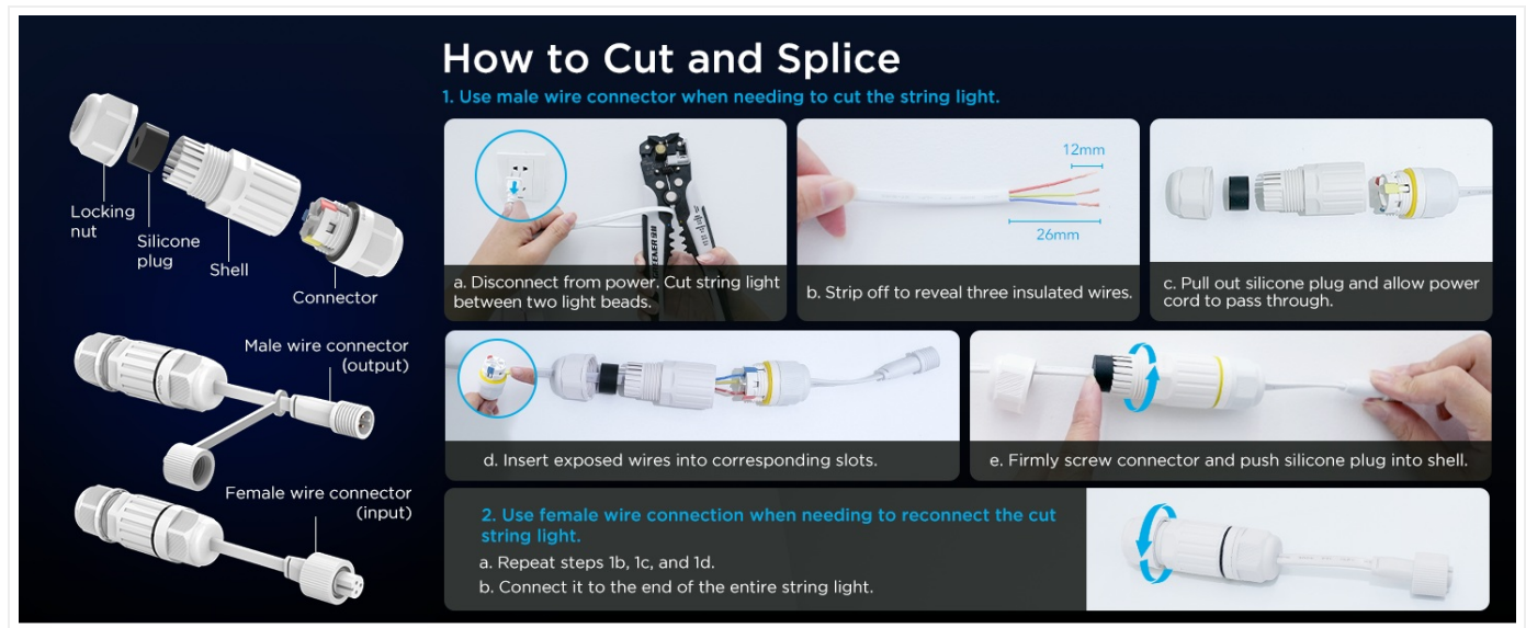
Image 4.1: Step-by-step guide on how to cut and splice the Govee Permanent Outdoor Lights Pro using male and female wire connectors.
