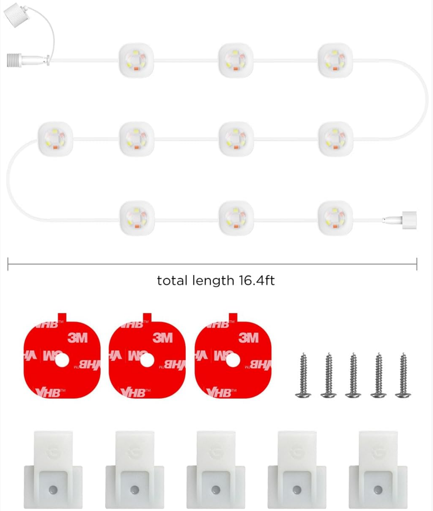
Image 3.2: Detailed view of the 16.4ft extension light strand, illustrating its length and the included installation accessories like VHB tape and clips.
