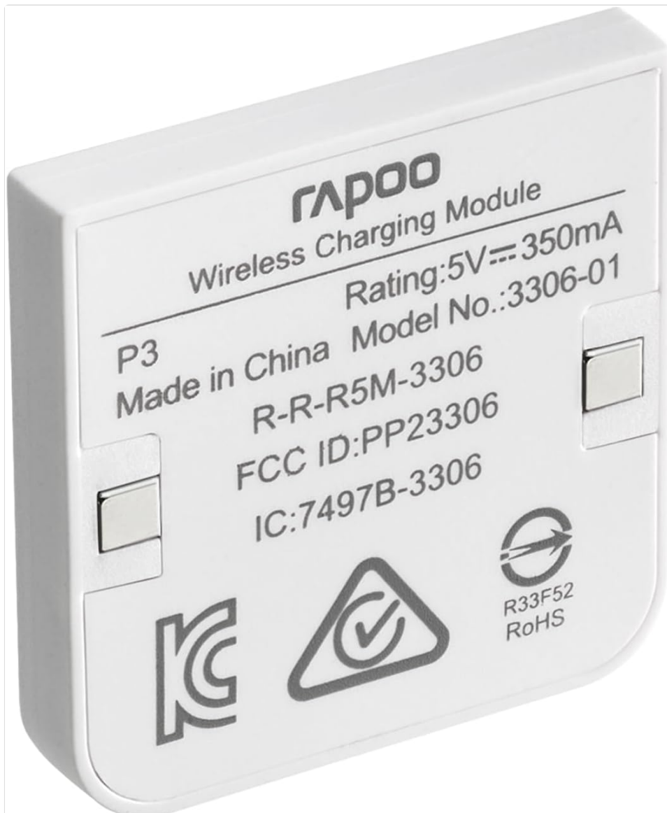
Image: Top view of the Rapoo P3 Wireless Charging Pack, showcasing its compact, white rectangular design.
