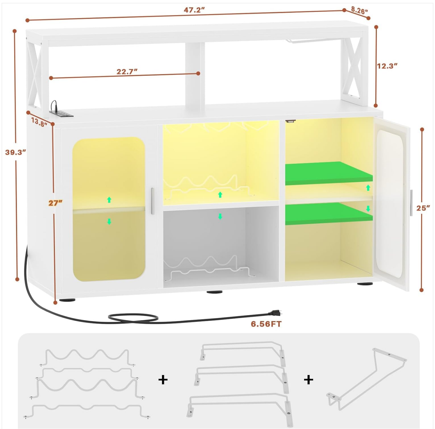
Figure 2.1: Exploded view and dimensions of the Aheaplus Bar Cabinet, including individual components like shelves, wine racks, and glass holders.
