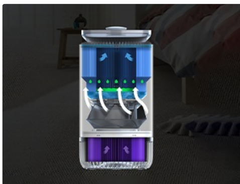
Image 5: Diagram showing the internal water circulation for the washing filter.
