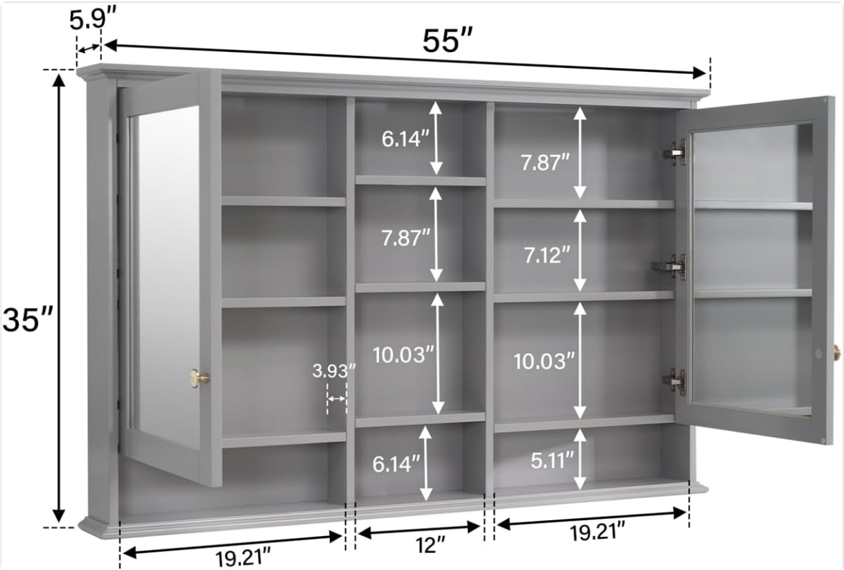
Image: Technical drawing illustrating the overall dimensions (55" W x 35" H x 5.9" D) and internal shelf measurements of the cabinet.
