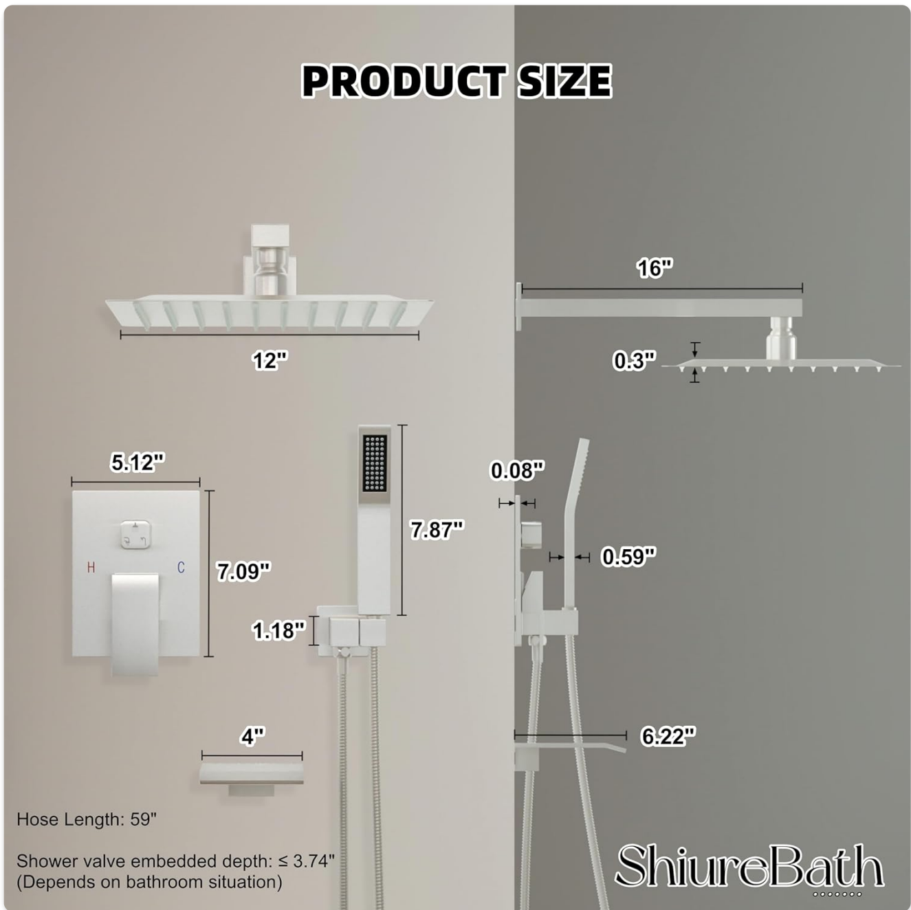
Image: A diagram illustrating the various dimensions of the shower system components, including the rain shower head, control panel, handheld shower, and tub spout.
