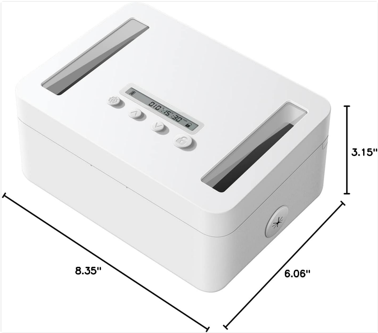
Image: Dimensions of the Vaydeer Metal Time Lock Box.
