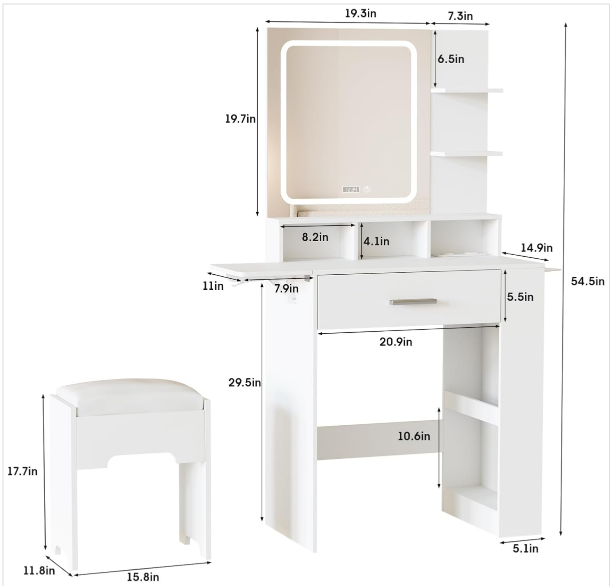
Image: Detailed dimensions and component layout of the Fameill Vanity Desk and accompanying stool.
