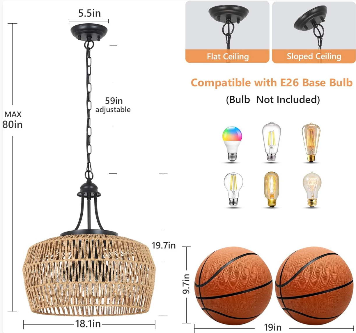
Image 3: Chandelier dimensions and bulb compatibility details.
