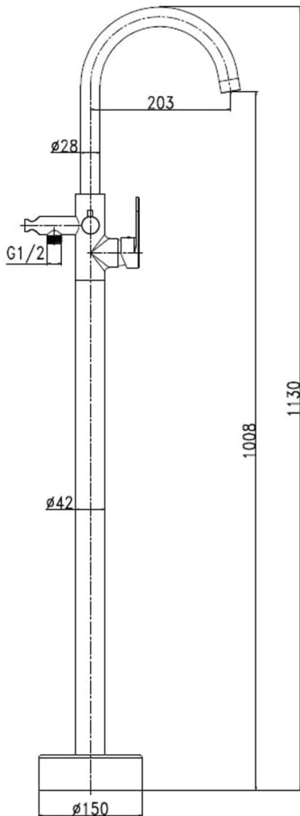
Image 2: Technical drawing with key dimensions.
