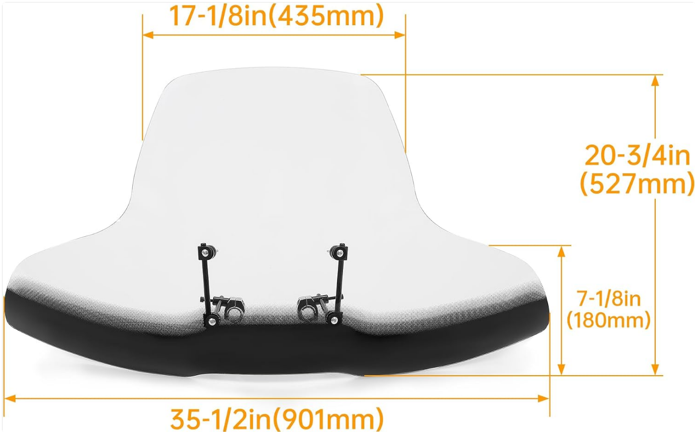
Figure 8.1: Product dimensions.
