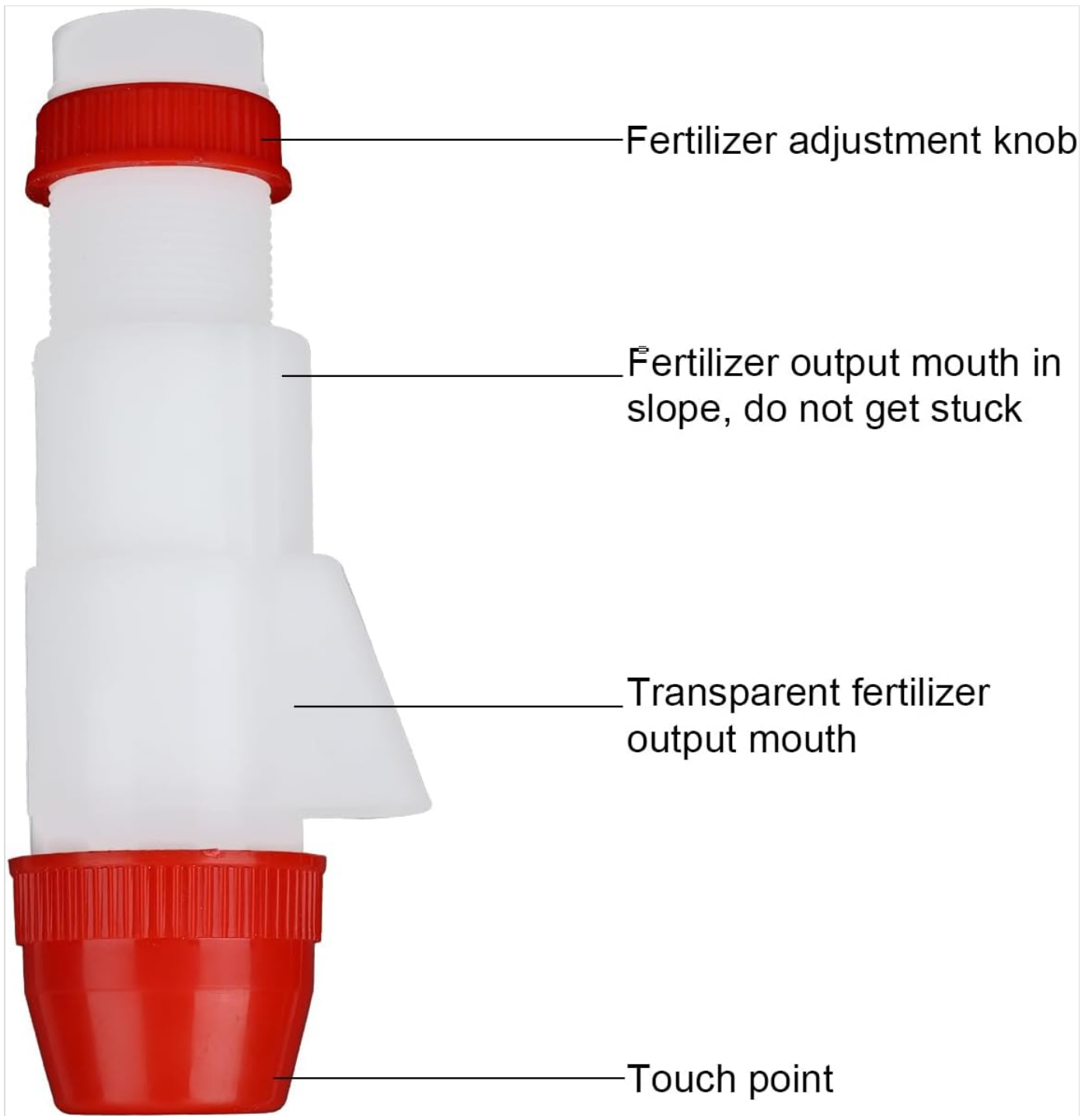
Figure 4.2: The fertilizer adjustment knob allows for precise control of fertilizer flow. The output mouth is designed to prevent clogging, and a transparent section allows monitoring of fertilizer flow.
