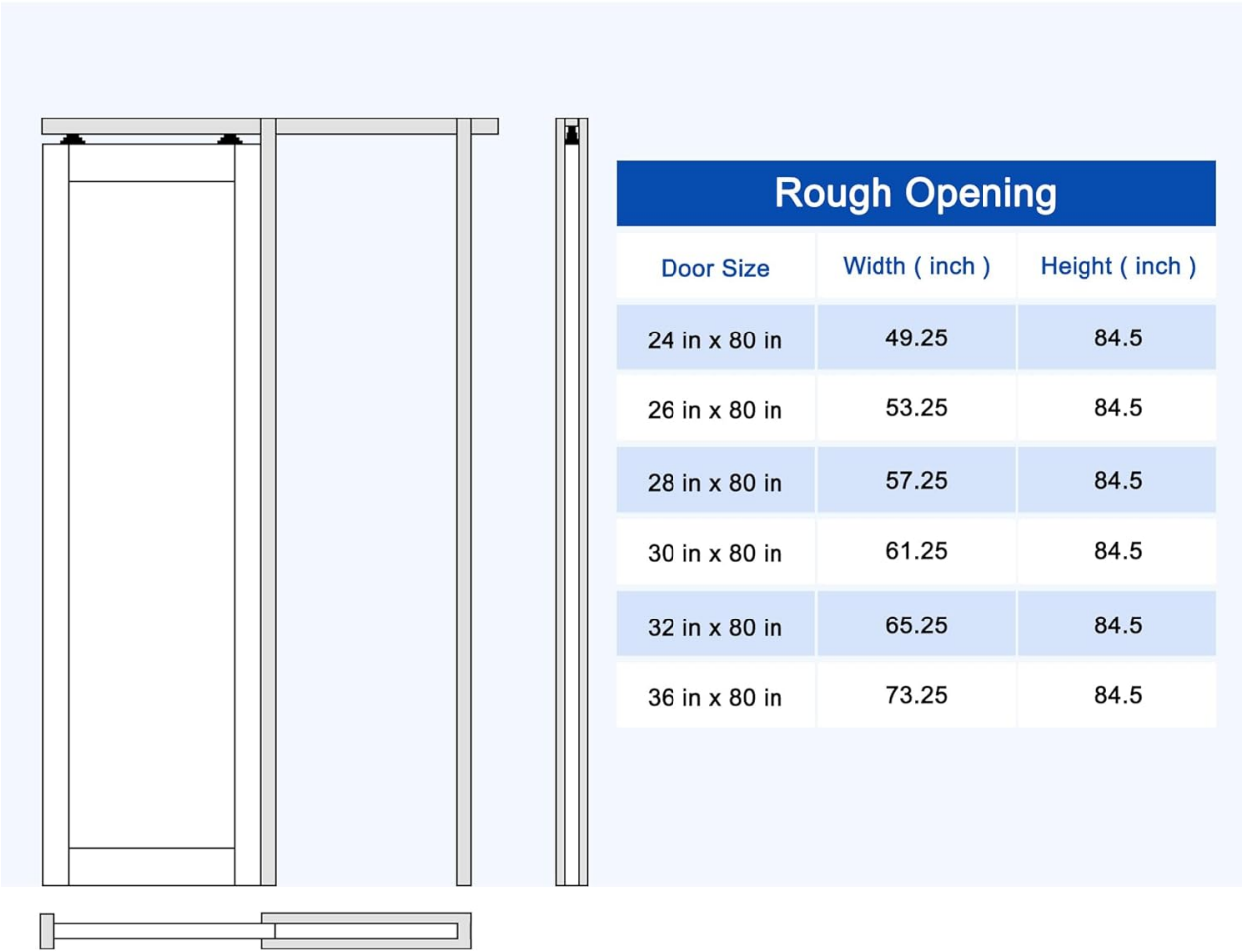
Image: A size chart illustrating the required rough opening dimensions for different pocket door sizes.
