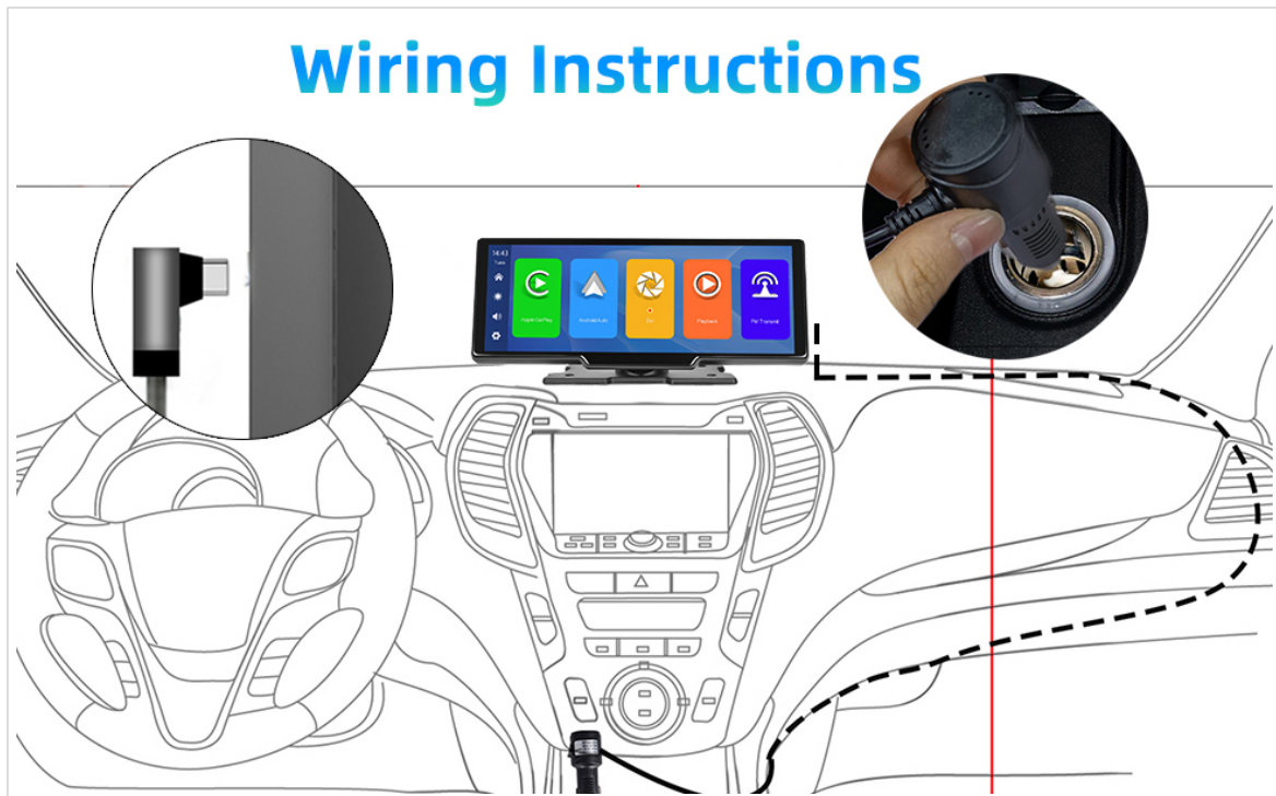
Image: Diagram illustrating how to connect the power cable from the multimedia player to the car's cigarette lighter socket and route the cable.
