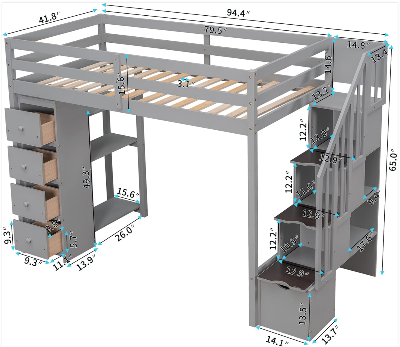
Image 5: Dimensional drawing of the Brabrety Twin Size Loft Bed, indicating length, width, and height measurements for all major components.
