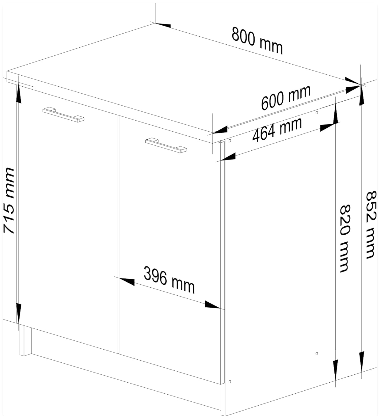
Image 4.1: Dimensional diagram of the AKORD Oliwia S80 Kitchen Cabinet. This illustration provides key measurements for planning placement and assembly.
