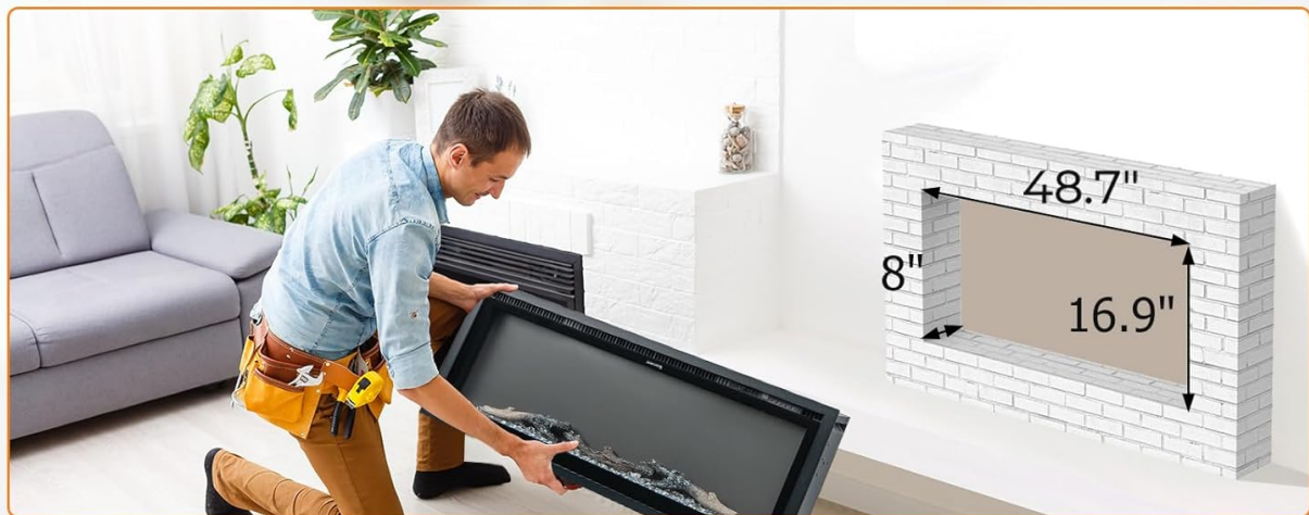
Figure 4.3: Detailed dimensions of the 50-inch fireplace and the required opening for recessed mounting.
