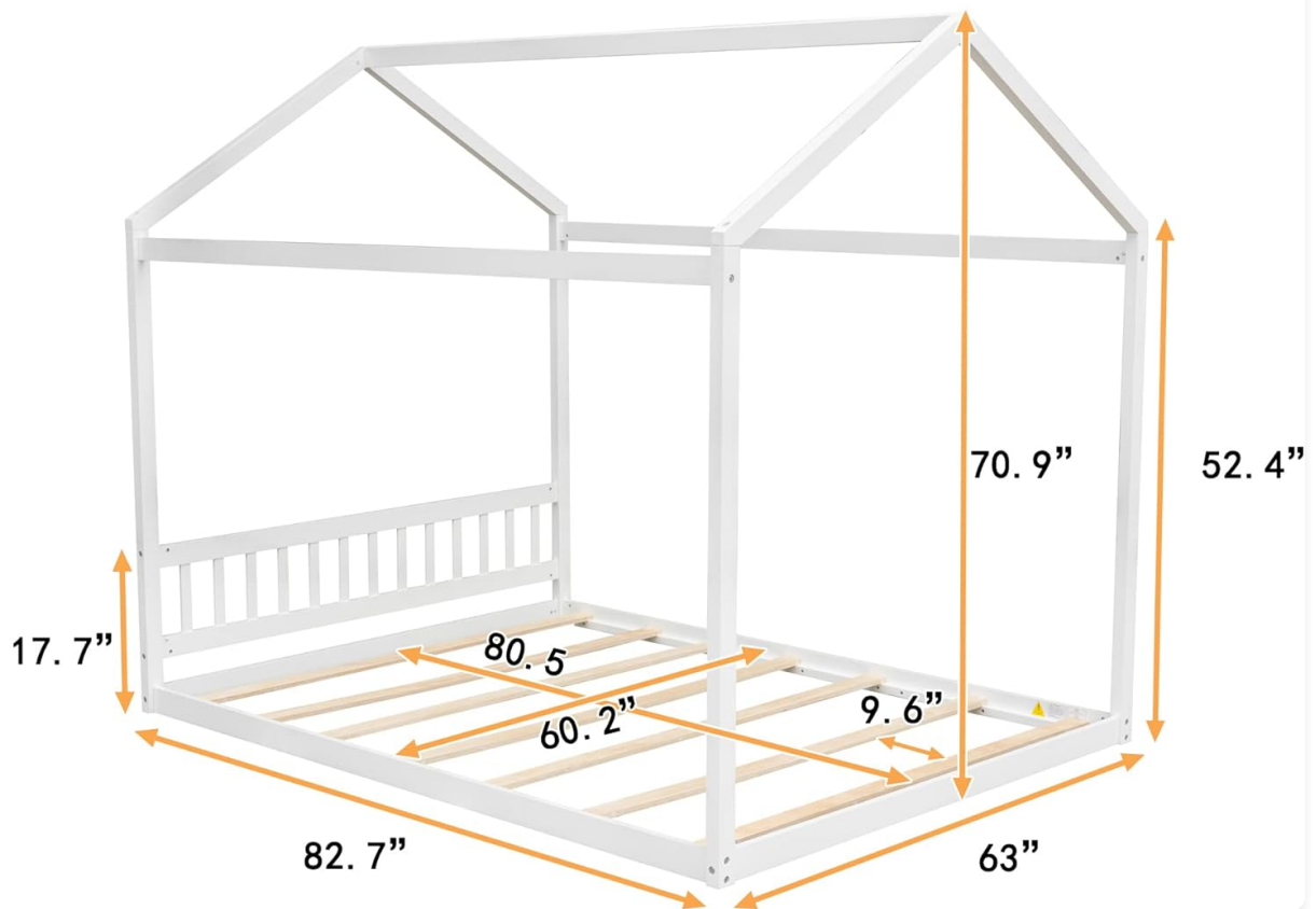
Image: Dimensional drawing of the Flieks Queen Size Wooden House Bed Frame, indicating length, width, and height measurements.
