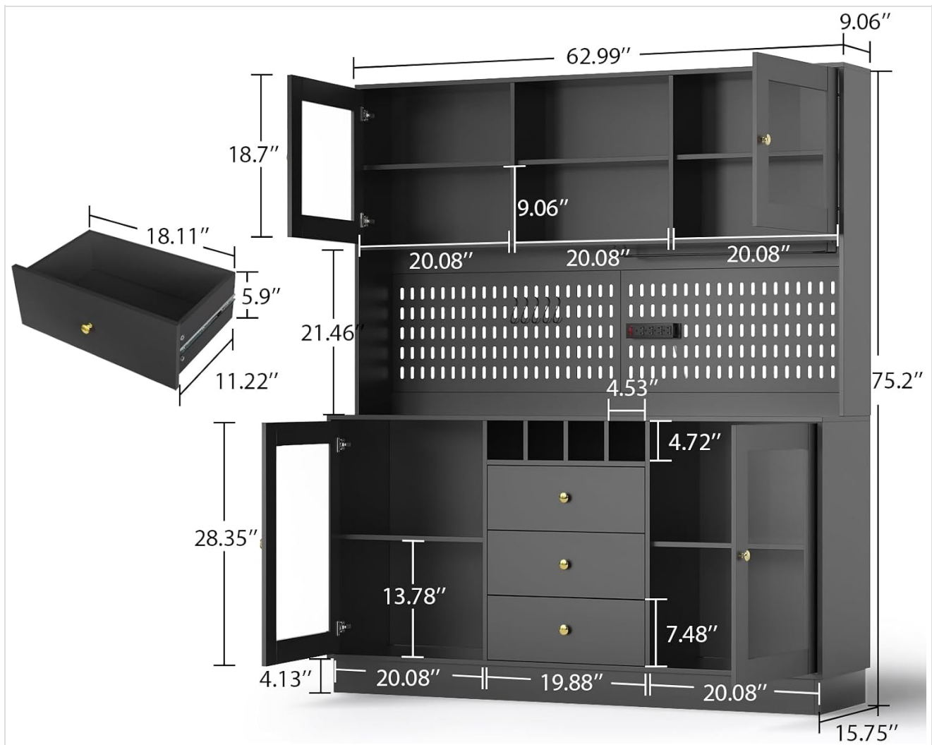
Figure 3.1: Product dimensions. Overall: 62.99"W x 15.75"D x 75.2"H.
