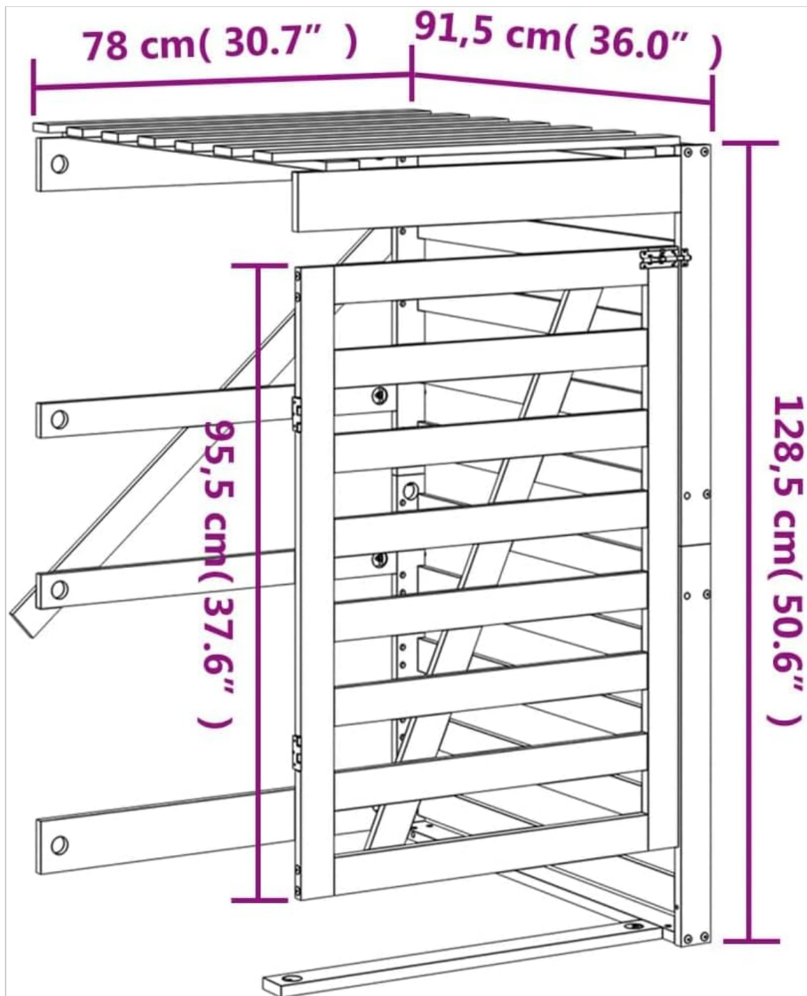
Image 6.1: Technical drawing illustrating the width, depth, and height dimensions of the storage extension.
