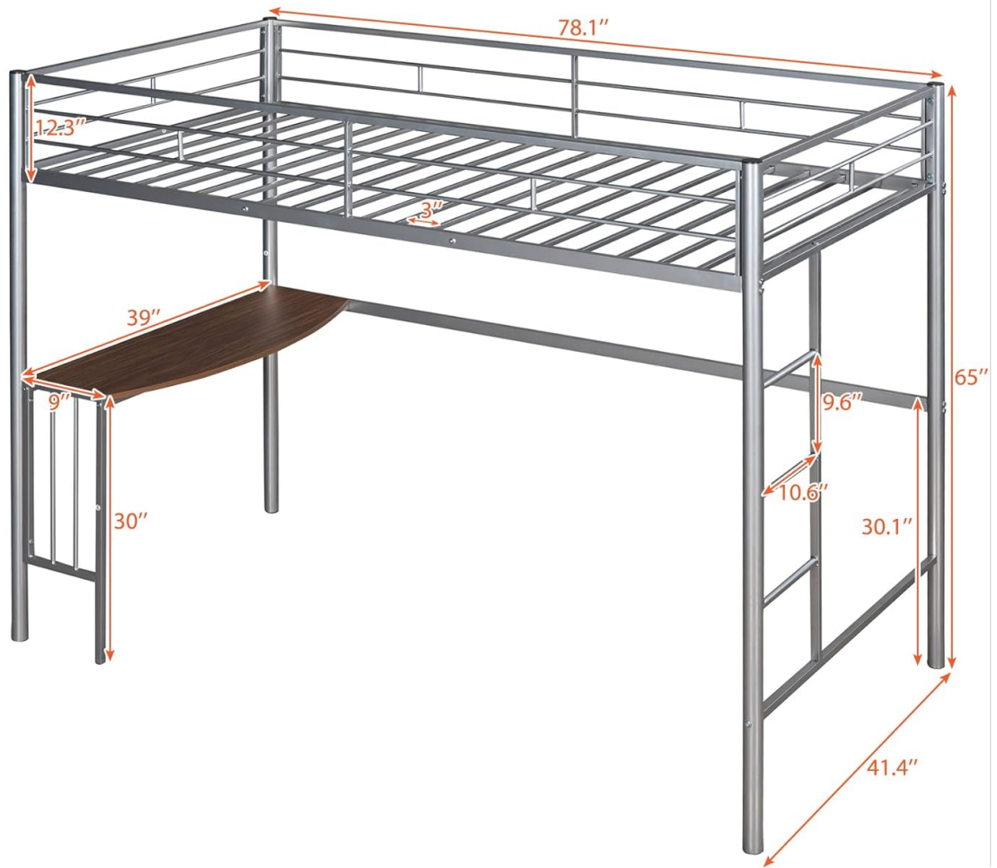
Figure 3: Side view illustrating the integrated desk and the ladder for upper bunk access.
