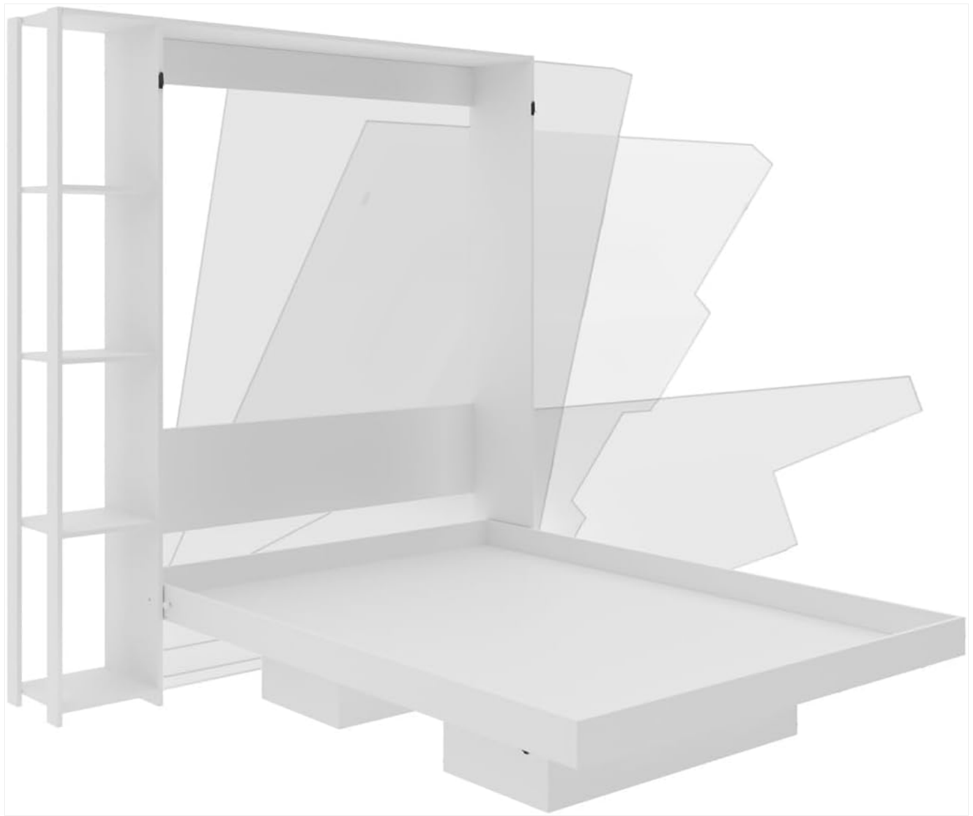
Figure 2: Assembly diagram and dimensions for the A22 CM8014.0101 bed base.
