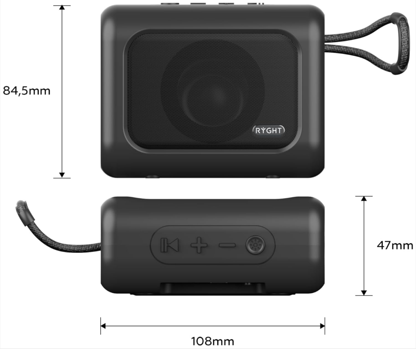
Image: Technical drawing showing the dimensions of the RYGHT QUBE speaker: 108mm in length, 84.5mm in height, and 47mm in depth.
