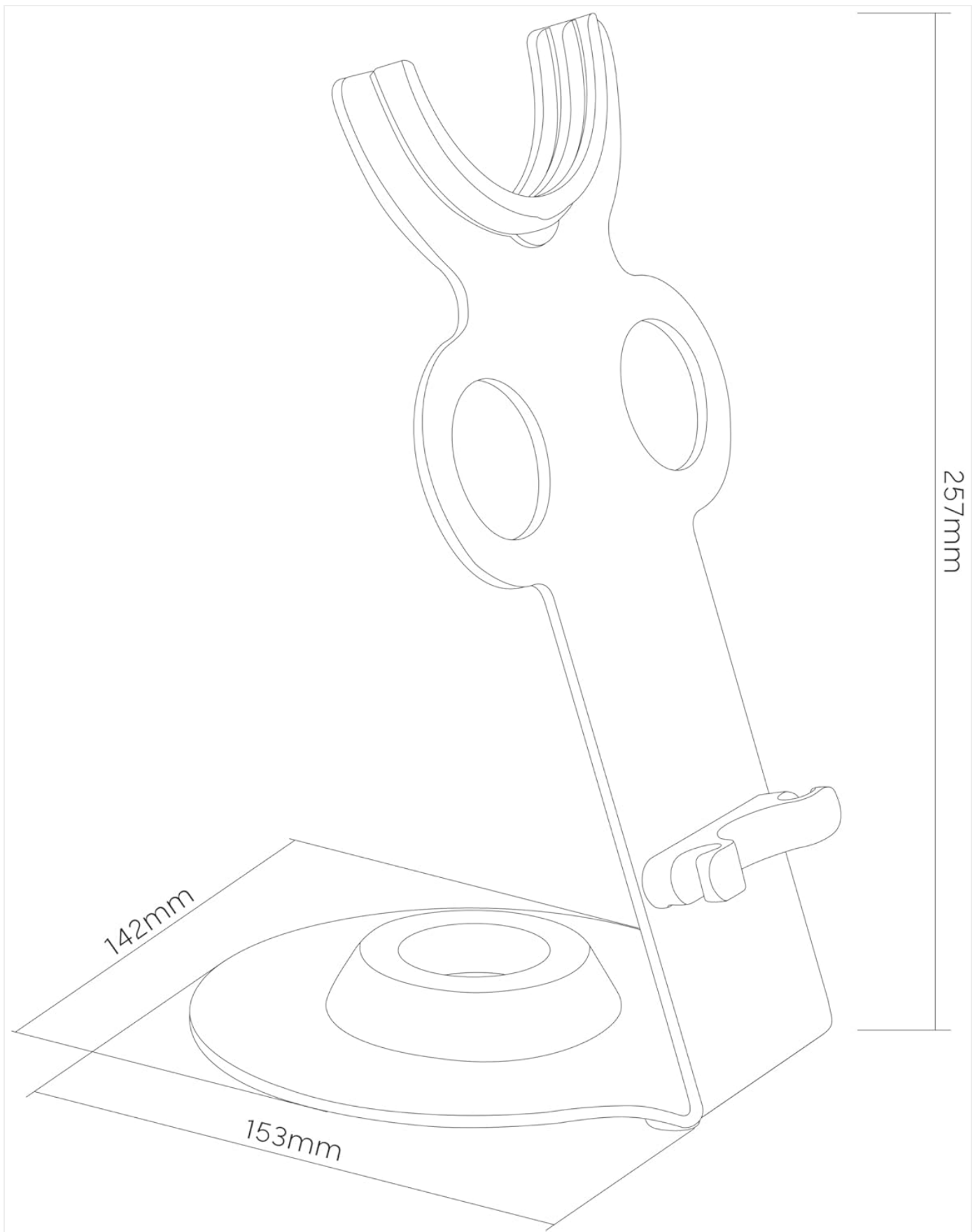
Image 8.1: Dimensional drawing of the stand, showing key measurements.
