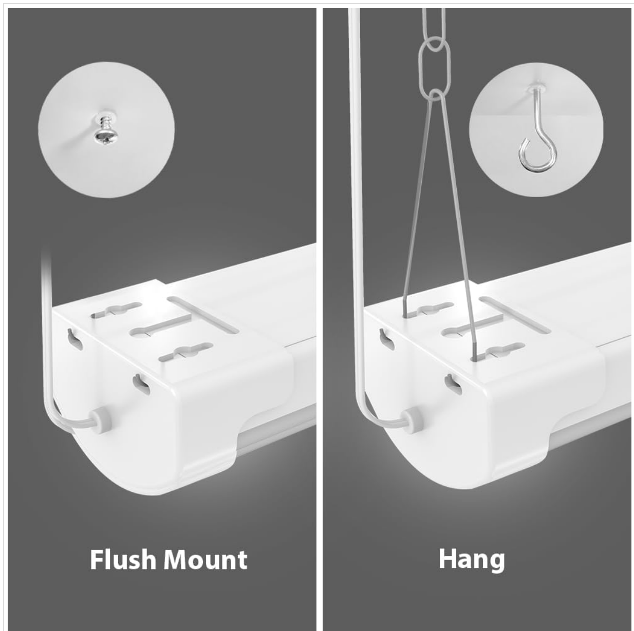
Image: A visual comparison showing how to perform a flush mount installation with screws and a hanging installation with chains and hooks.
