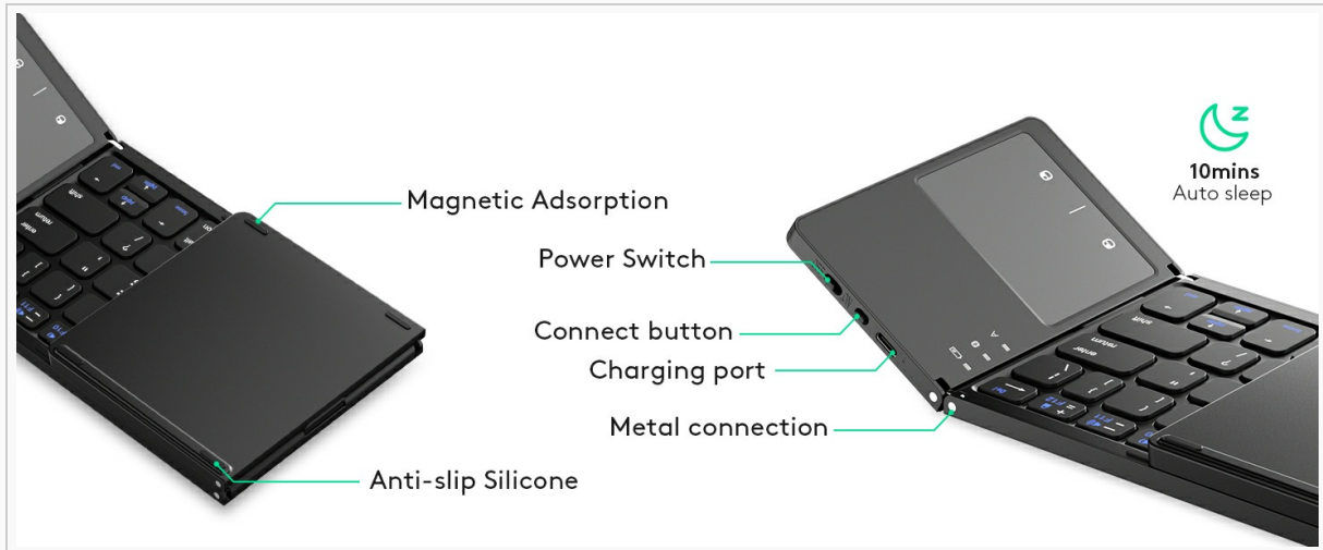
Image: A detailed view of the keyboard's side, highlighting the Power Switch, Connect button, and Charging port.
