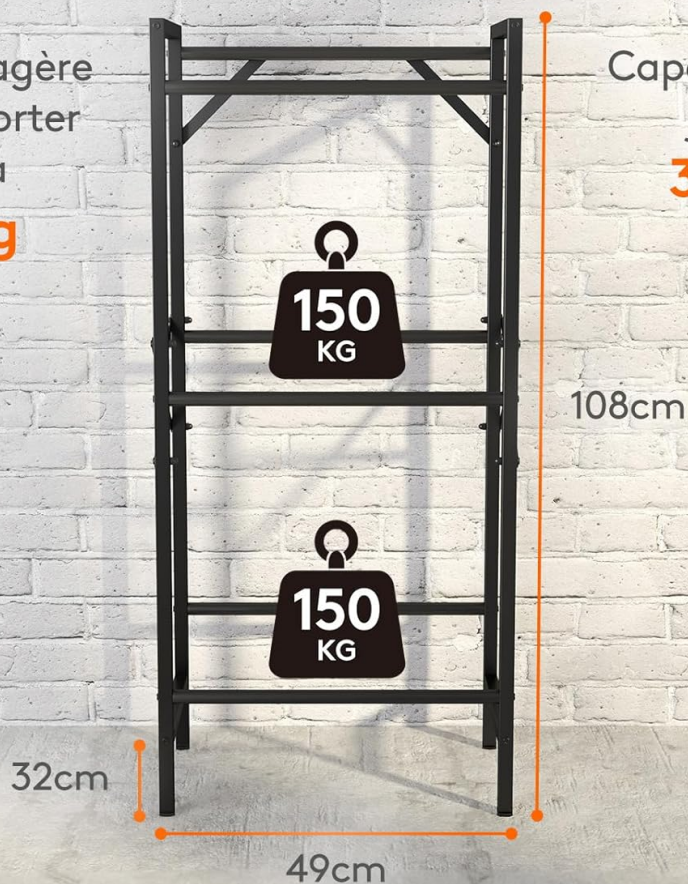
Image 5.1: Load capacity and dimensions of the Lifewit Beverage Crate Rack.
