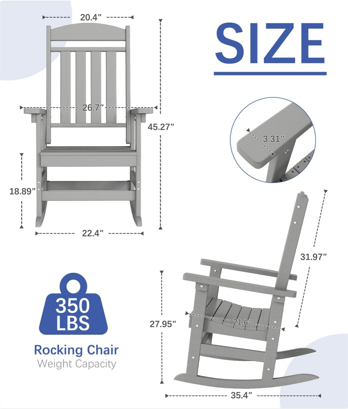
Image: Detailed dimensional drawing of the FOOWIN rocking chair, including height, width, depth, and seat depth.
