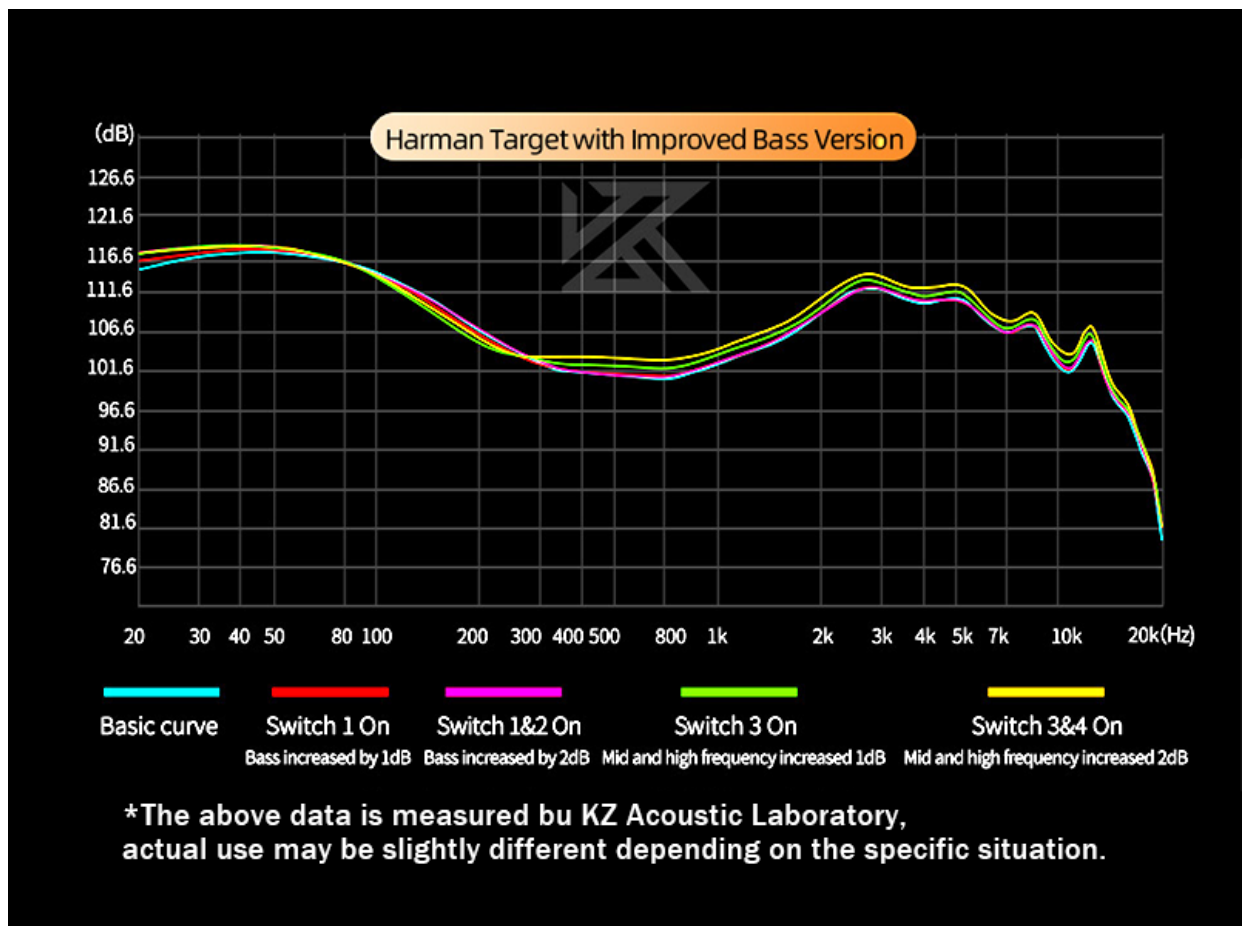
Image: A frequency response graph illustrating how different combinations of the tuning switches alter the sound profile of the KZ Castor earbuds.
