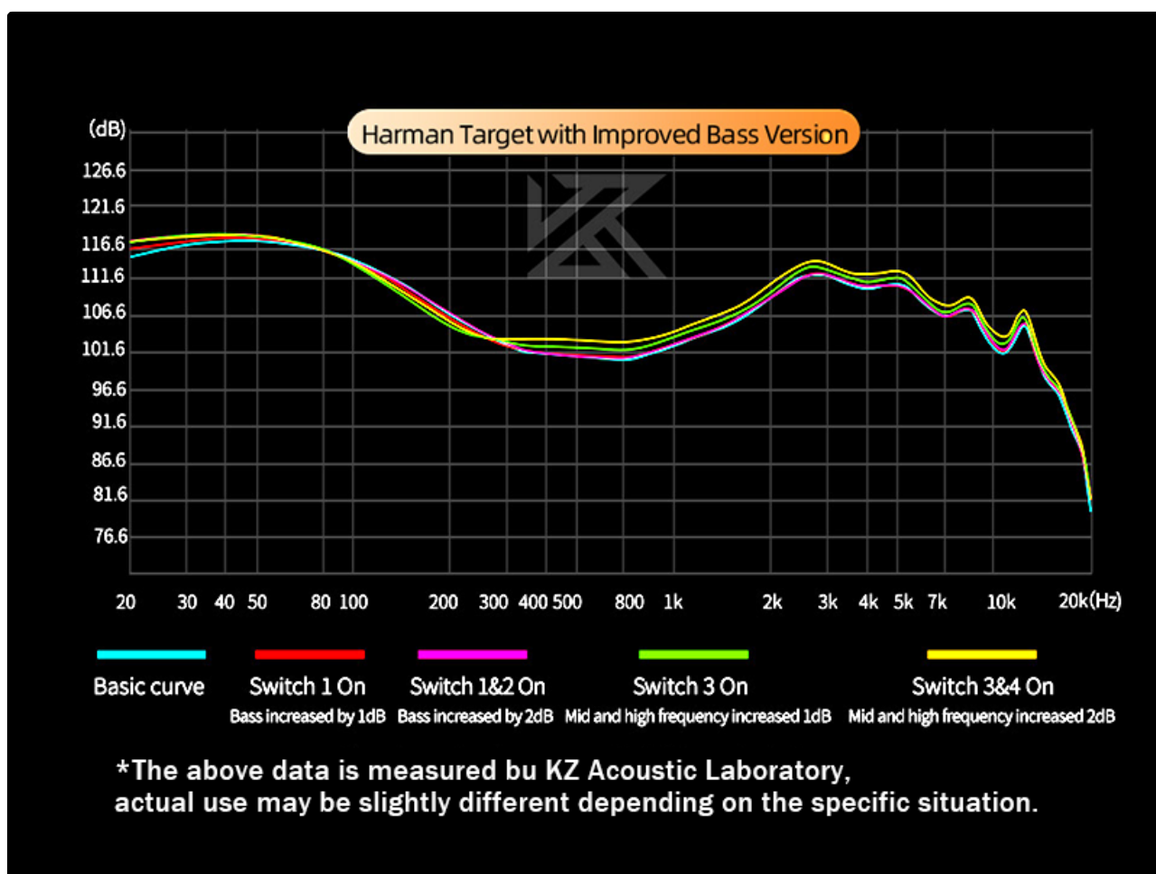
Image: Frequency response graph illustrating the impact of different tuning switch combinations on the KZ Castor's sound profile.
