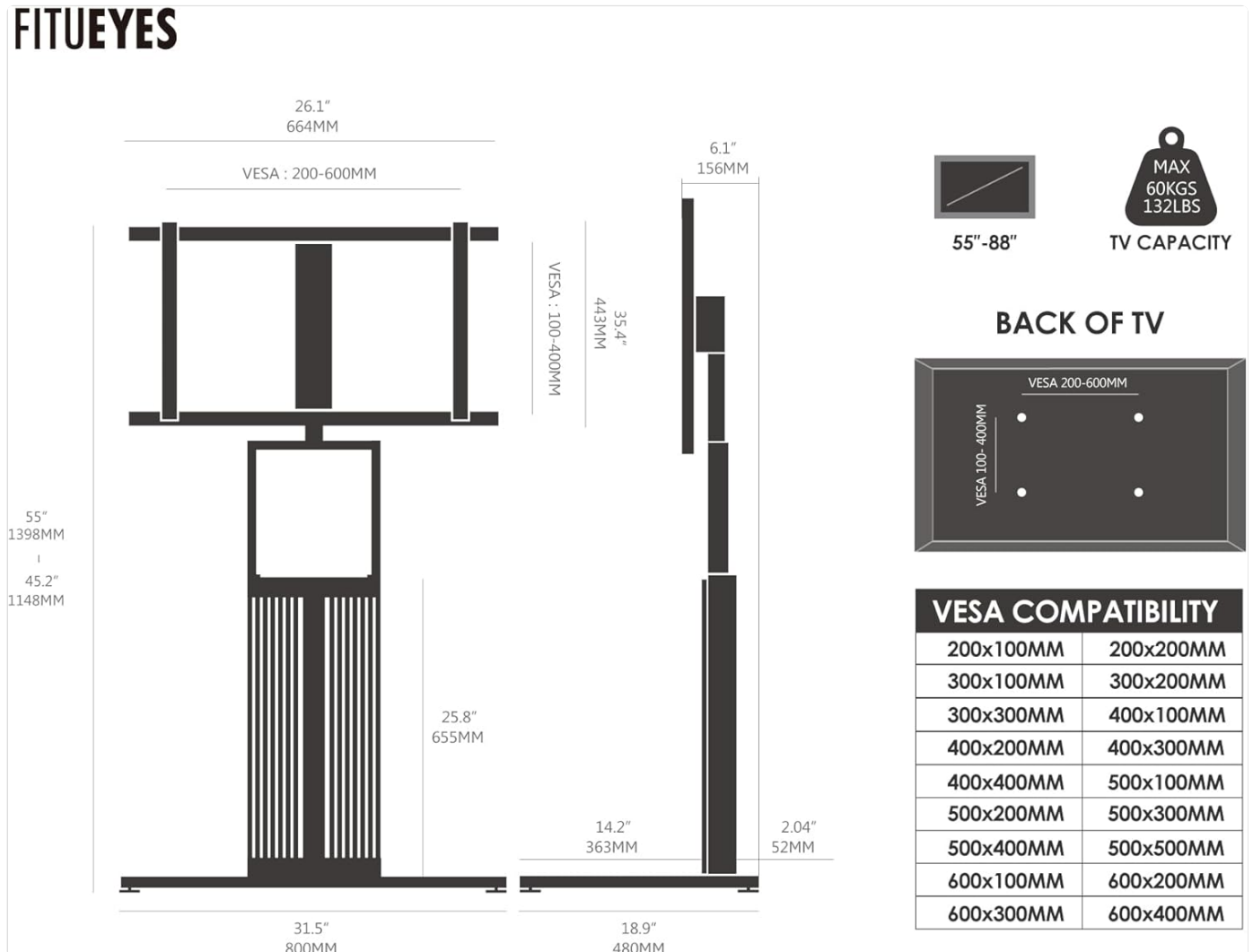
Image 4.3: VESA compatibility and stand dimensions diagram.
