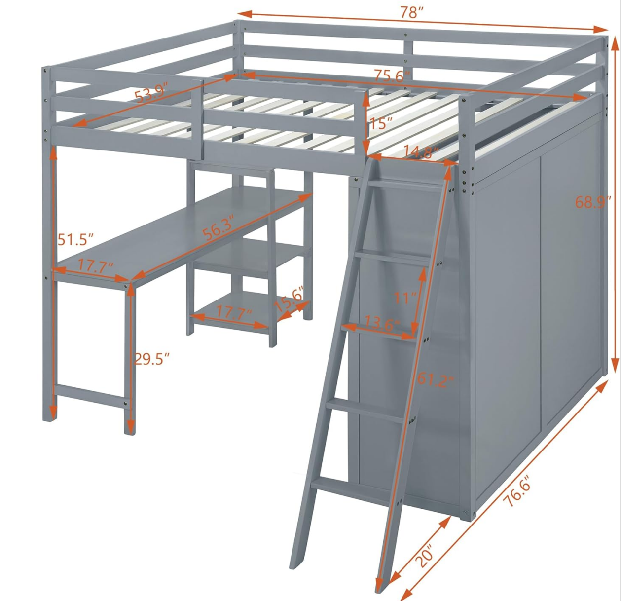
Image 9: Angled dimension diagram, illustrating overall length, width, height, and specific measurements for the desk, bed platform, and ladder.
